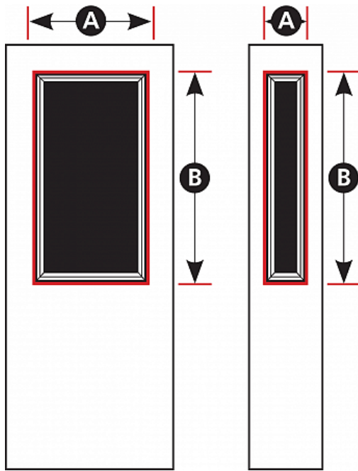
Half-view Door and Sidelight
